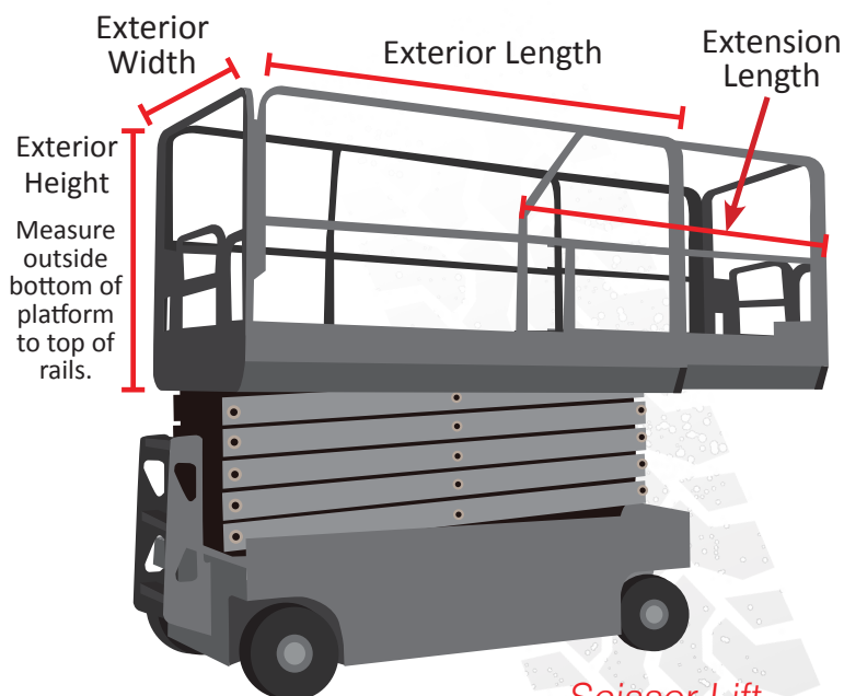
Scissor Lift
