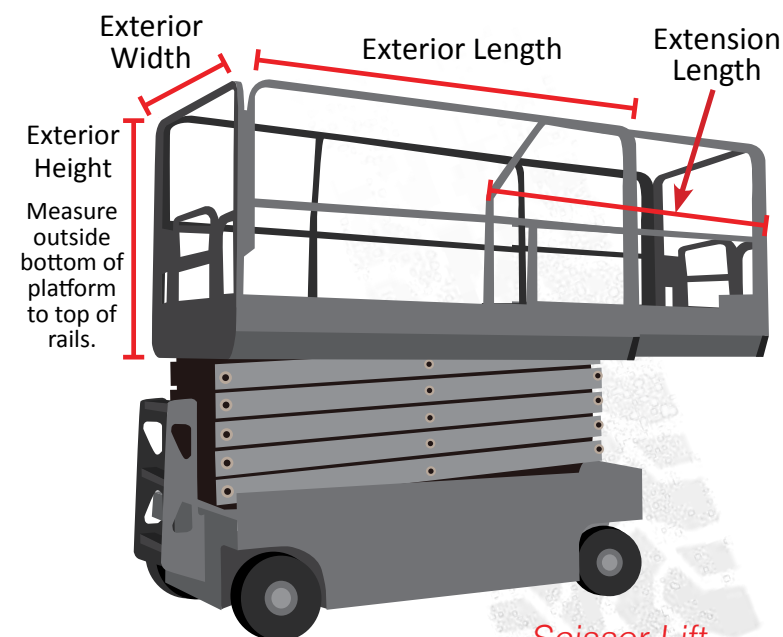
Scissor Lift
